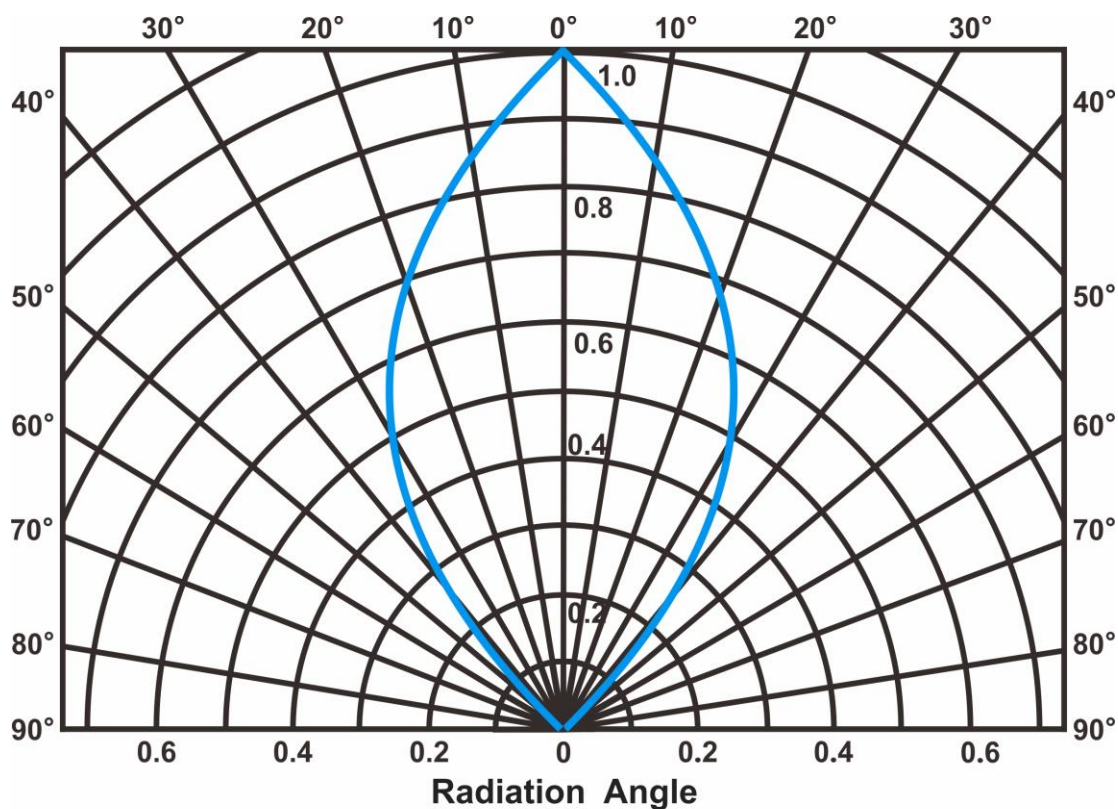
Radiation Characteristics
