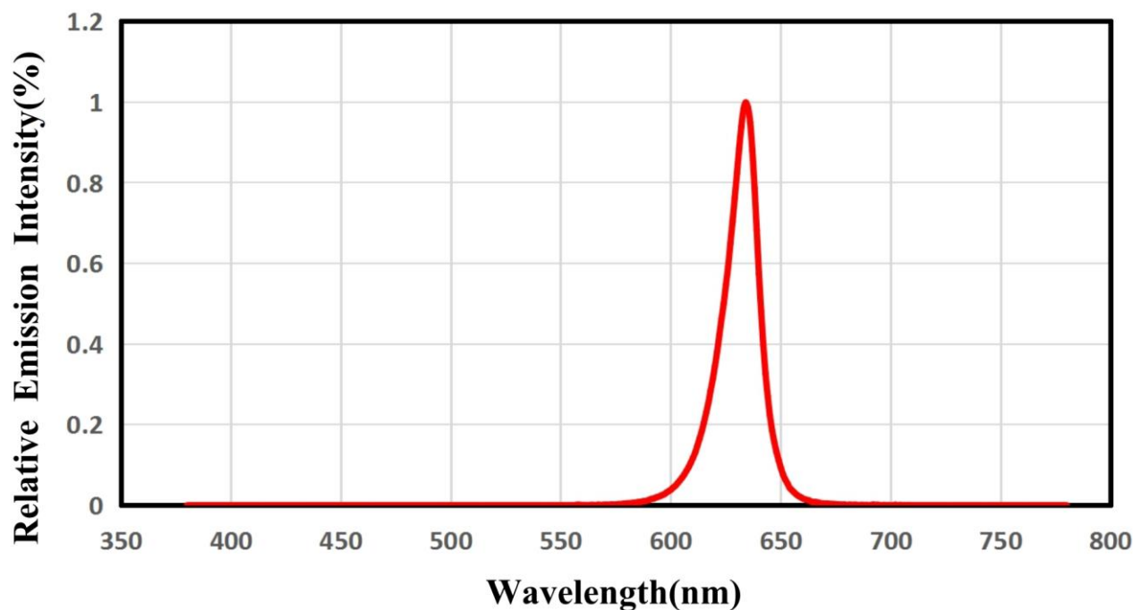
Radiation Characteristics
